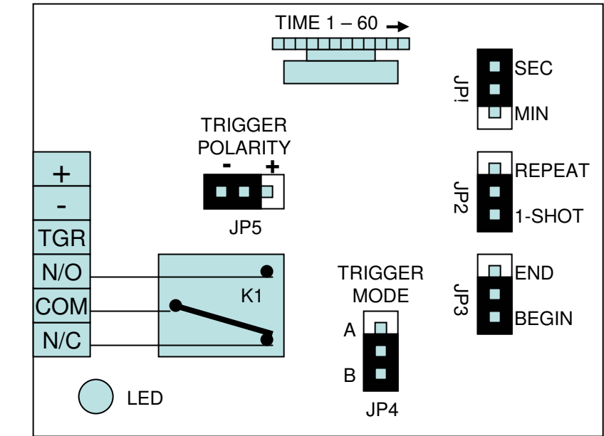
Serial Port Interface Timer Board
